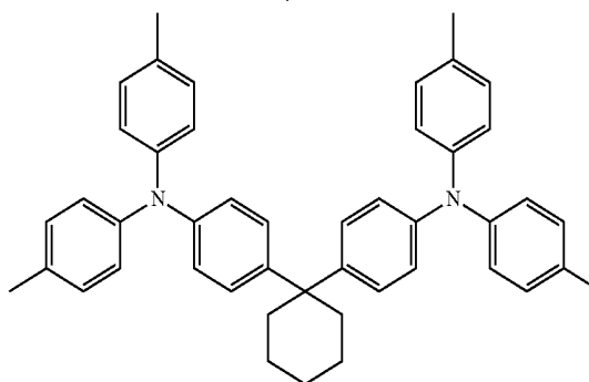
methylated NPB
