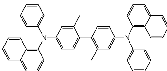
Spiro-NPB
