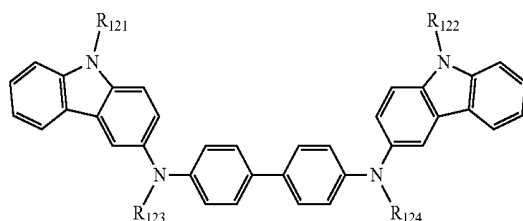
Formula 202
