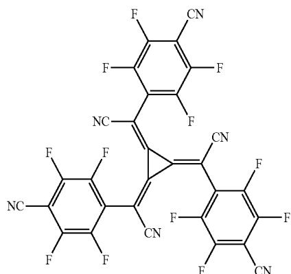
Compound HT-D2
