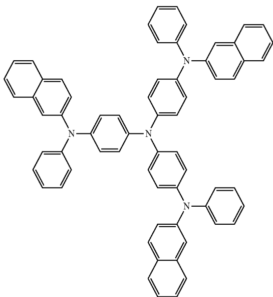
2-TNATA
