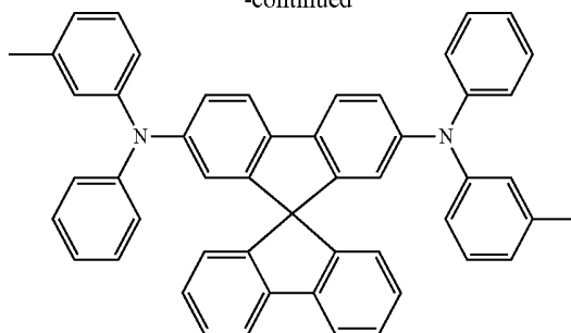
Spiro-TPD
