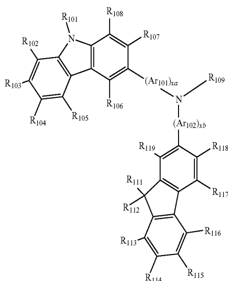
Formula 202
